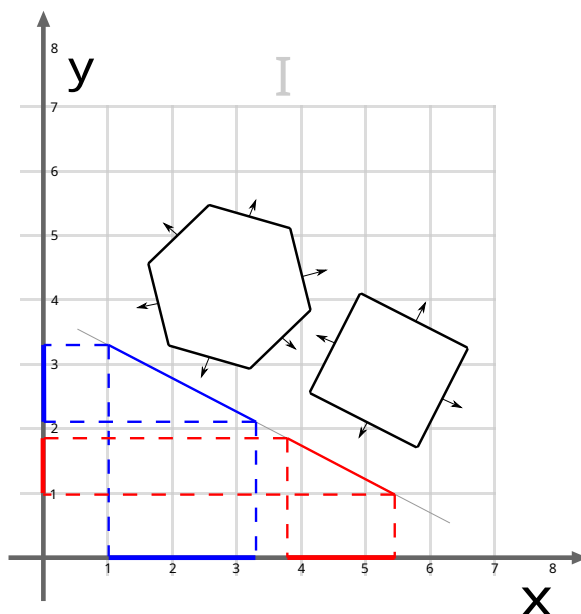
Figure 204: Projecting our projections onto the x and y axes
